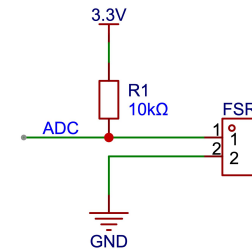
Figure 11: Voltage Divider Circuit: This simple voltage divider circuit converts the resistance change of the FSR sensor into an analog voltage on the ADC line.
